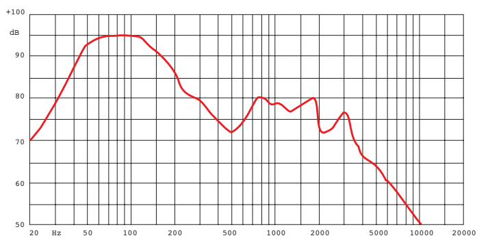
Frequency response B 12 B 1W/1m (full space)
