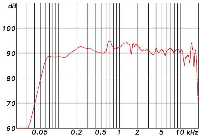
F 8 Sens. 2,83V/1m: 91,3 db (100-10k) 57 Hz - 18,5 kHz (-6 dB)
